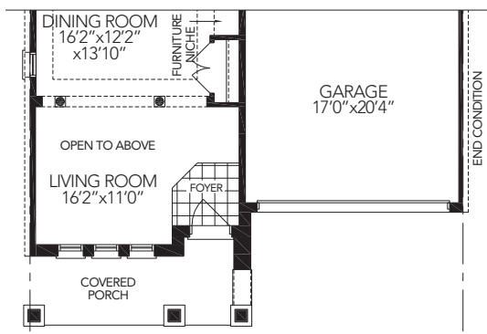
PARTIAL GROUND FLOOR ELEV. B
